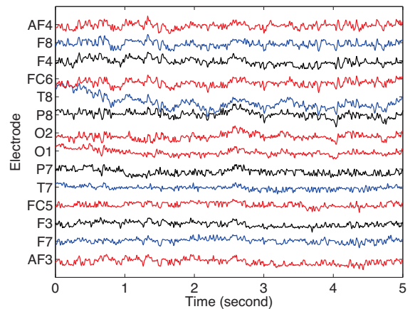
Figure 3: Raw data from the headset
