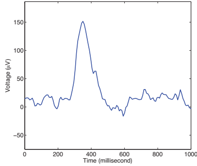
Figure 5: Unfiltered wink signal from one electrode. The difference from the peak of the wink signal to the background noise is about 140\mu V
